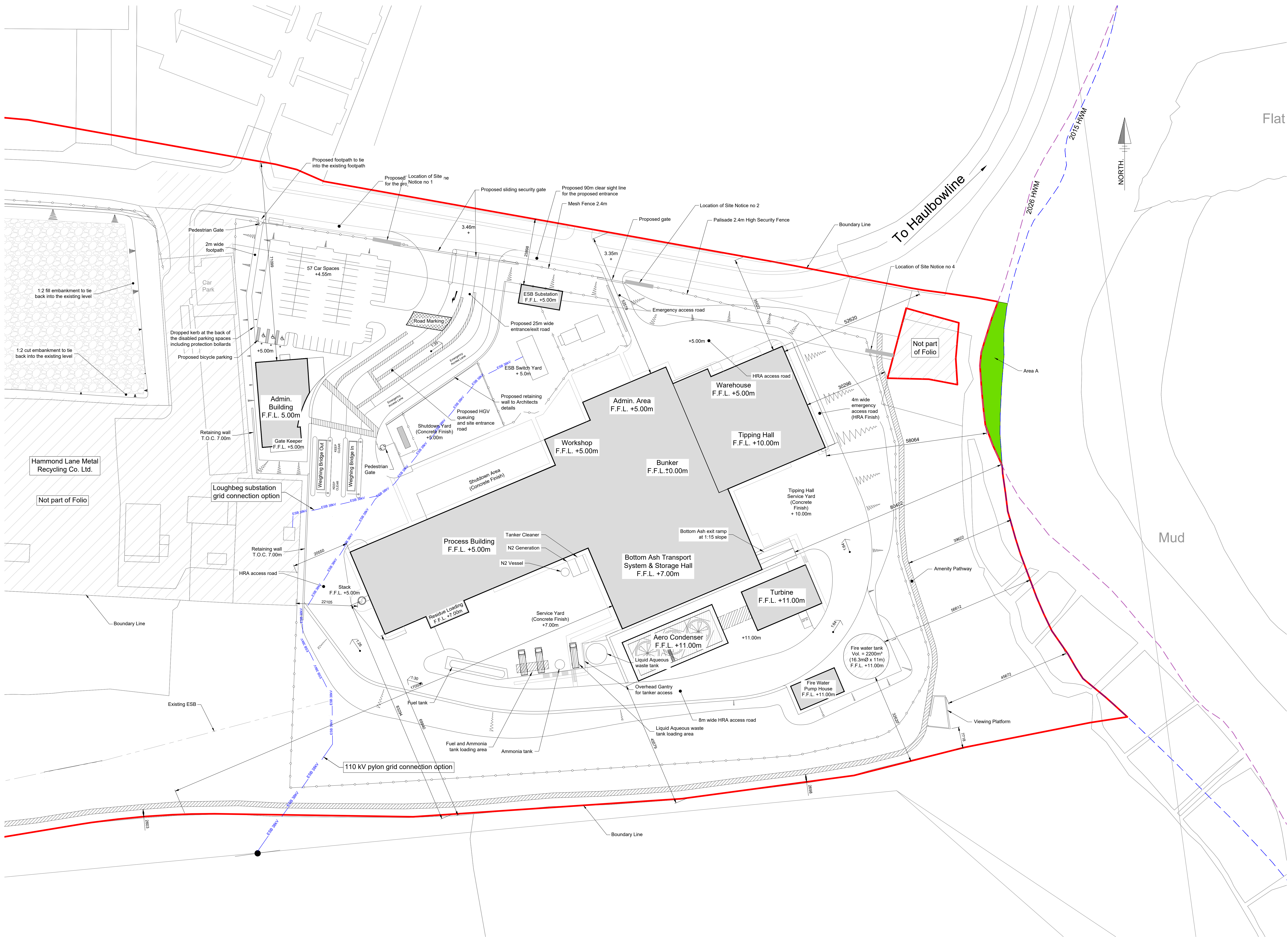
PROPOSED SITE LAYOUT PLAN - 2026 (SCALE 1:500 @A0)
